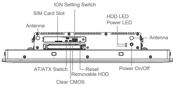
Front I/O
